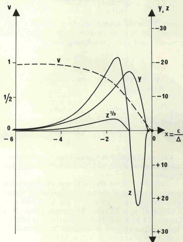
FIGURE 6 The functions y , z , z^{1/3} and v versus the parameter x = \epsilon/\Delta for 2\Gamma_0/\Gamma_1 = 10.4 .
